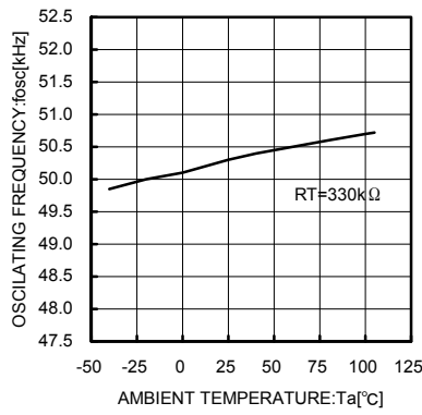
Fig.2 Frequency vs. Ambient temperature (All series)
